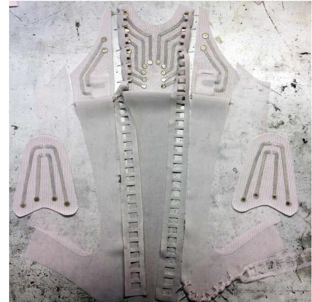
Figure 5 Toile #2: Second Skin pattern piece layout showing assembled eTextile panels and laser cut ladders to house tubing for cables
