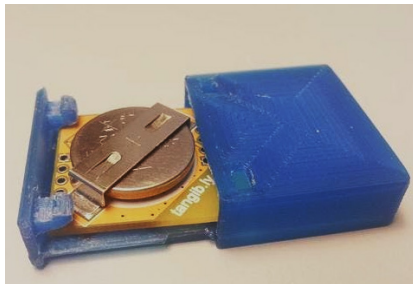
Figure 4 – Twiz (Tiny, Wireless, IMUz) in 3d printed enclosure.
